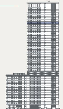
EAST ELEVATION
